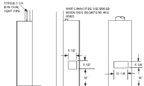
WHEN SIDE REGISTERS ARE NOT USED UNIT MAY BE RECESSED UP TO 9 1/2"
